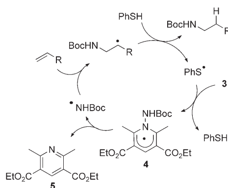
Scheme 1. Radical transfer hydroamination with 3 using polarity-reversal catalysis (PRC).
