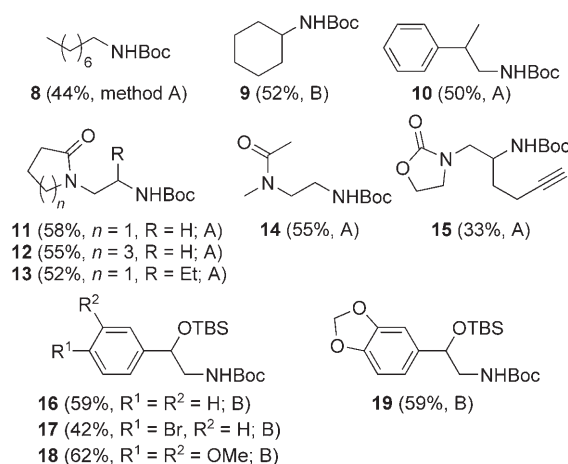
Figure 1. Hydroamination of various olefins. Reaction conditions: benzene (0.4 M), olefin (2–10 equiv), reagent 3 (1 equiv). TBS = tert -butyldimethylsilyl.
