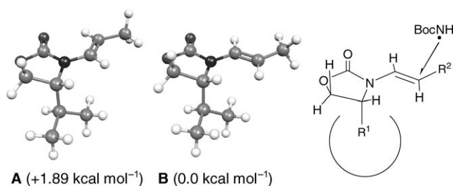
Figure 3. Conformers A and B of ent - 20i and model to explain the stereoselectivity. The energy difference mainly results from dipole interactions of the C=O and C=C bonds.
