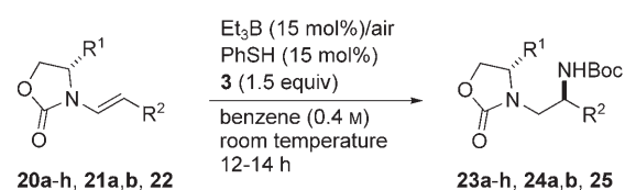
Scheme 3. Stereoselective radical transfer hydroaminations. R 1 and R 2 are specified in Table 2; only the major isomer of the product is shown.
