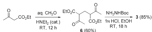
Scheme 2. Synthesis of hydroamination reagent 3 .
