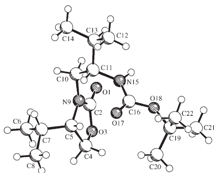
Figure 2. Molecular structure of the major isomer of the protected 1,2-diamine 23c .
